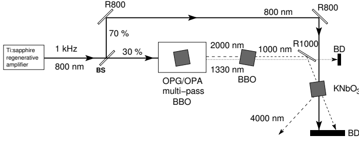
FIGURE 2.1. Generation of femtosecond pulses with a wavelength around 4000 nm for time-resolved non-linear spectroscopy. Legend: BBO, \text{KNbO}_3 : crystals; R800, R1000: dielectric 800 nm, 1000 nm mirrors; BD: beam dump; OPG/OPA: three-pass optical parametric generation and amplification stage based on BBO.
