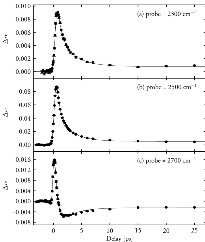
FIGURE 4.6. Pump-probe delay scans of a diluted solution of HF in pyridine at different probe frequencies with a pump frequency tuned to 2500 cm -1 . The solid line is calculated using a model which is described in §4.4.2.
