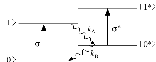
FIGURE 6.4. States and decay scheme used to describe the relaxation of the excited C–O stretch vibration. The cross sections for a radiative transition are indicated by \sigma and \sigma^* . The rate of the 1 \rightarrow 0^* relaxation is given by k_A and the rate of the 0^* \rightarrow 0 relaxation is given by k_B .
